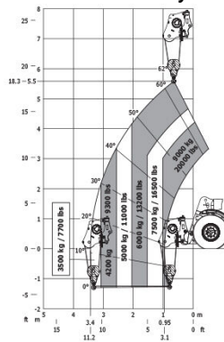
Machine on tyres with winch Metric
